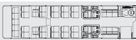
35' Low Floor 33 + 2 Wheelchairs or 41 Passengers
