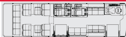
30' Low Floor 24 + 2 Wheelchairs or 30 Passengers
