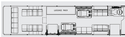
35' Low Floor 22 + 2 Wheelchairs or 28 Passengers
